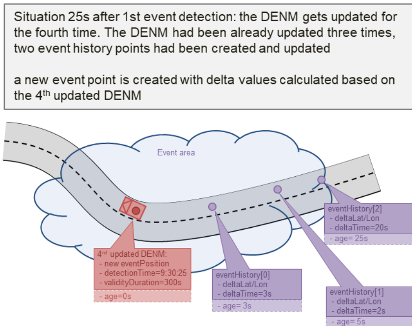
Figure 3 (h) - Generation and evolution of eventHistory along an event area
